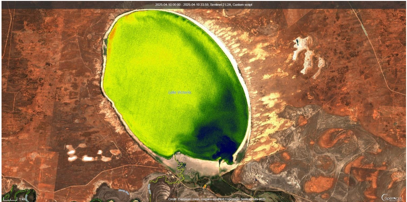
Figure 4: Lake Victoria 15/04/2025 SentinelHub [CC BY-NC 4.0] NSW-Custom Algae Script - TF, WaterNSW.
