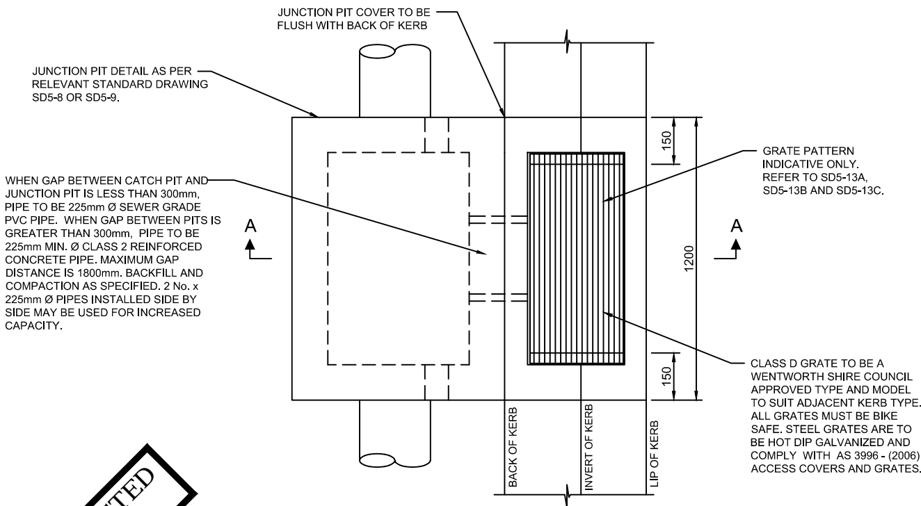
GRATED KERB CATCH PIT WITH CORBELLED JUNCTION PIT
