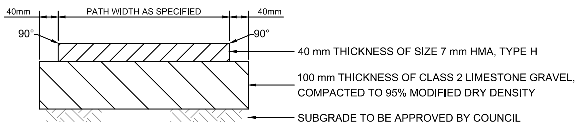
TYPICAL PAVEMENT SECTION NOT TO SCALE
